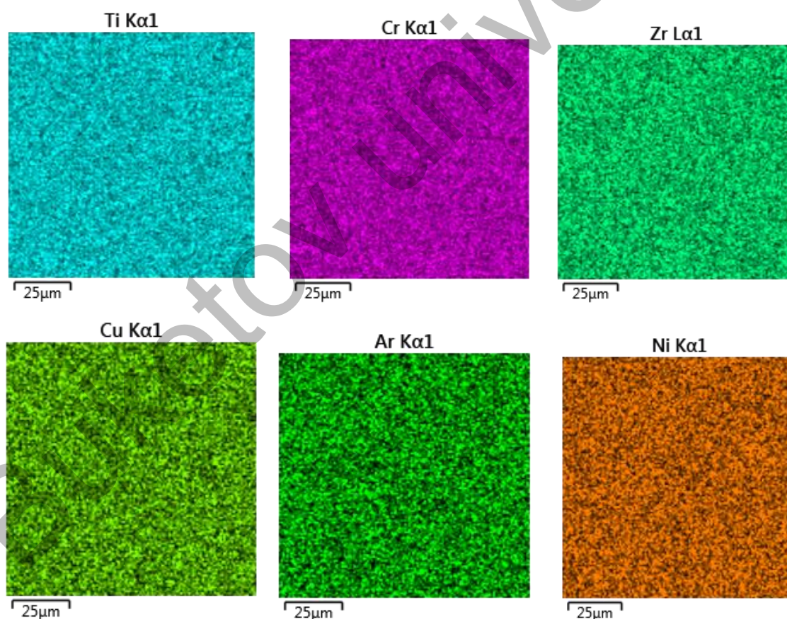
Fig.6. Distribution of TiNiZrCuCr elements deposited on 12X13 steel in argon
