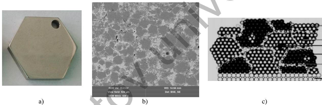
Fig.3. A sprayed sample with an HEC-coating (a), an REM image of an HEC-coating (b), a diagram of the formation of nanostructured coatings of an HEC-coating [17].
