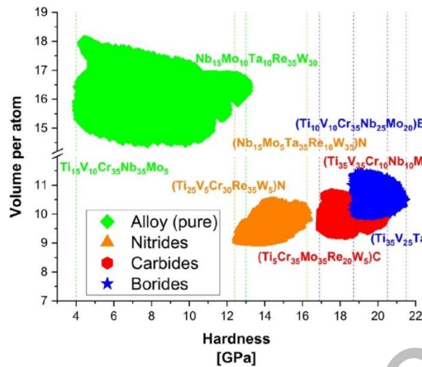
Fig.1. Graphical representation of predicted hardness of high-entropy alloys and compounds based on the refractory metals: dotted lines represent the maximum and minimum hardness [11].
