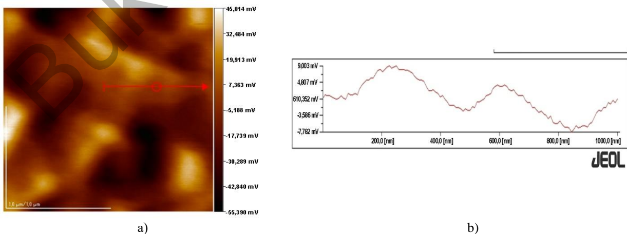
Fig.4. AFM image of TiNiZrCuCr (a) and its roughness (b), [18].
