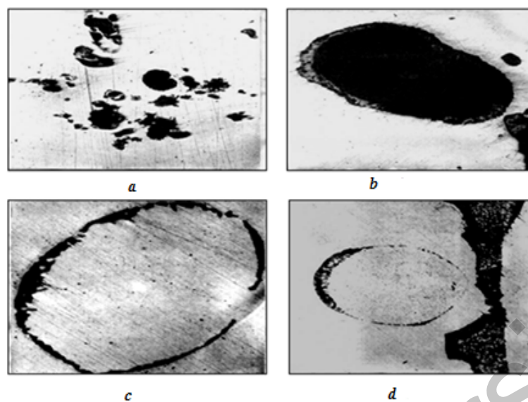
Fig.5. Microstructure of the ingot corner templates: a) x 50; b) x100; c) x 500; g) x200; a), b) are gas bubbles in the cortical zone of the ingot; c), d) are bubbles filled with metal with an oxide shell.
