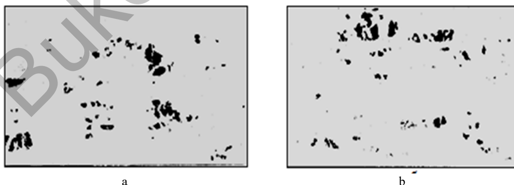
Fig.2. Microstructure of steel at the location of the defect: a, b - nonmetallic inclusions in a cold-rolled sheet along the surface of the sheet (x 400);
