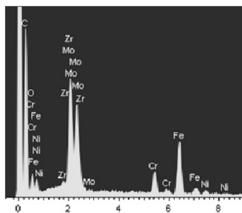
Figure 4b. Energy Dispersive Spectrum of a Section Sample Cross Section
