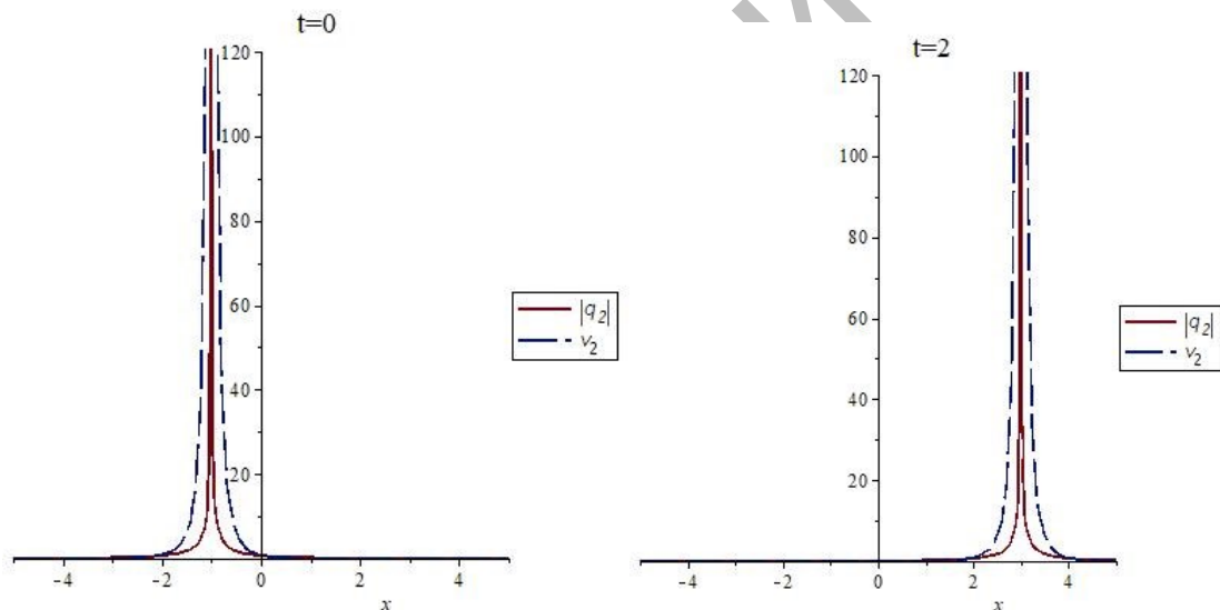
Fig. 6. The 2D-graphs of the solutions q_2 (solid line), v_2 (longdash line) with the parameters a = 1, b = 1, d = 2
