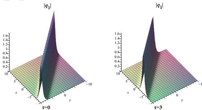
Fig.1. The 3D-graphs of the solution q_1 when a = 1 , b = 1 , d = 2
