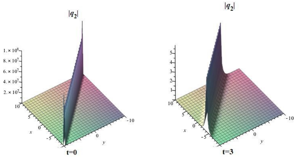
Fig.3. The 3D-graphs of the solution q_2 when a = 1, b = 1, d = 2
