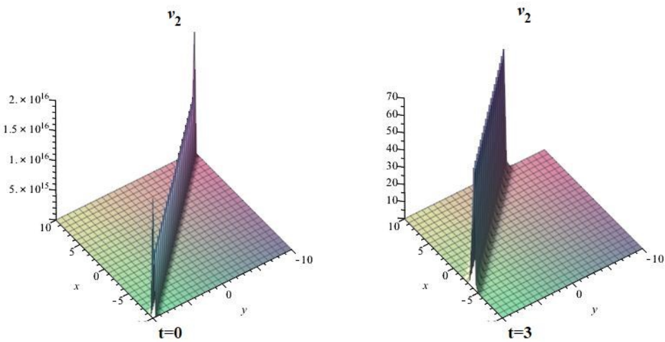
Fig. 4. The 3D-graphs of the solution v_2 when a = 1, b = 1, d = 2
