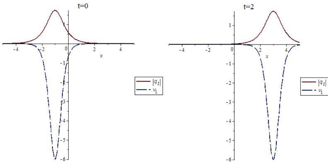
Fig. 5. The 2D-graphs of the solutions q_1 (solid line), v_1 (longdash line) with the parameters a = 1, b = 1, d = 2
