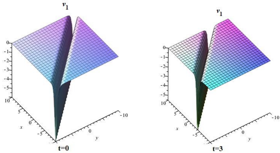
Fig. 2. The 3D-graphs of the solution v_1 when a = 1, b = 1, d = 2
