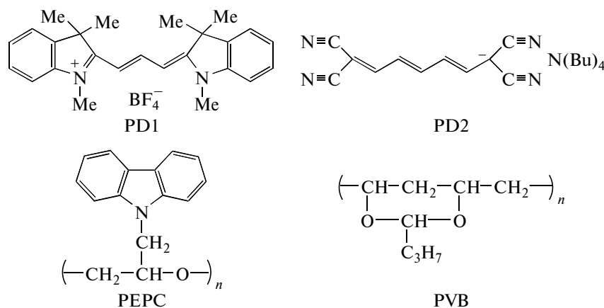
Fig. 1. Structural formulas of PD1 and PD2 molecules and PVB and PEPC monomer units.
