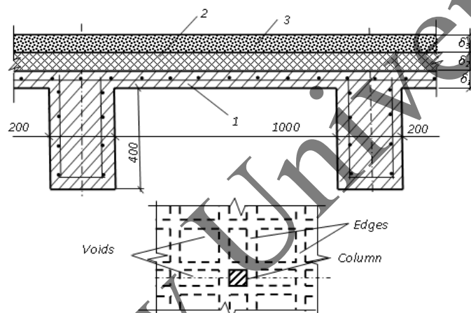
Fig.4. Pan floor: 1– heavy layer concrete; 2 – a layer of heat-insulation material; 3 – top protective layer.
