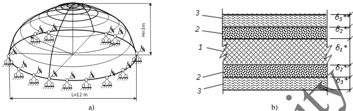
Fig.3. Five-layer model for the shell: a) shell structure; b) the structure of a five-layer material (1 – central layer; 2 – middle layers; 3 – surface layers).
