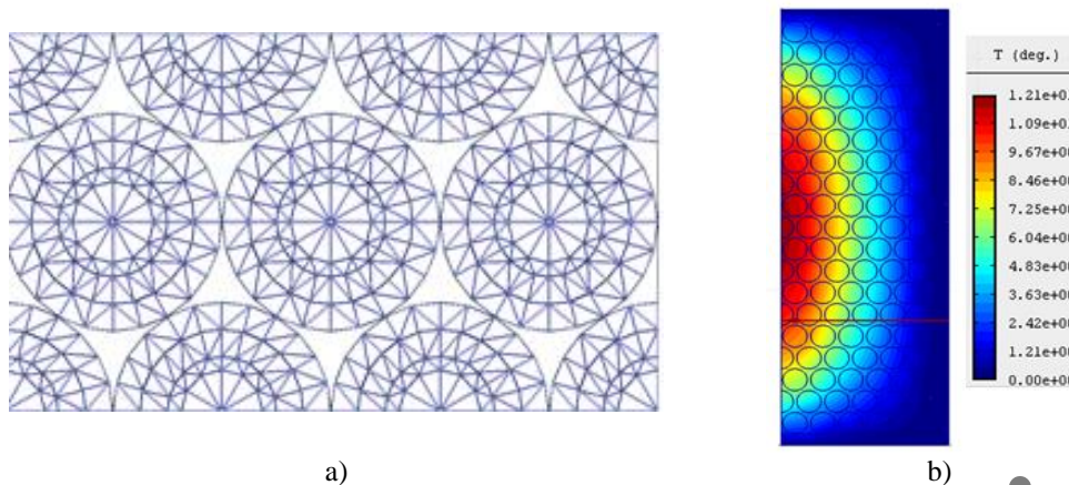
Fig.1. Model of a composite material with regular packing of granules of the same diameter: a) layout of filler's particles; b) temperature fields obtained in the Agros2D program.
