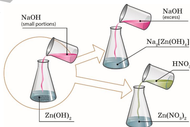
a — extraction of zinc hydroxide; b, c — dissolution of the precipitate Zn(OH)_2
