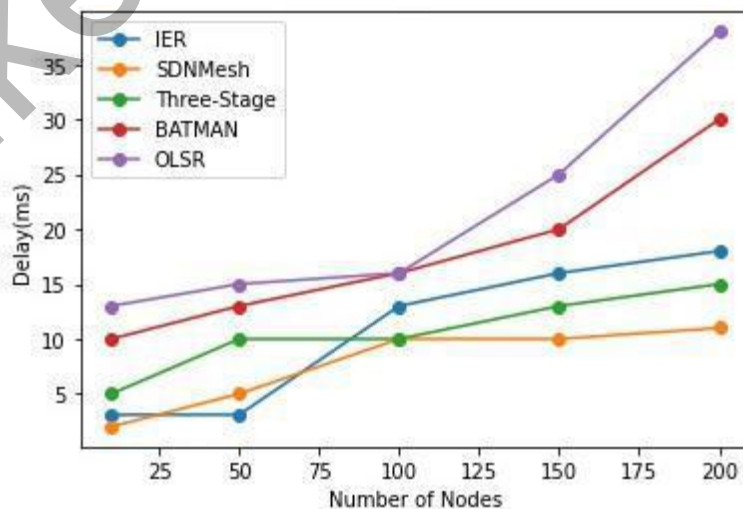
Fig.5 Deley.
