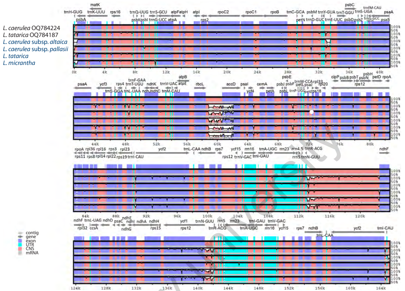
Fig. 2. Comparison of complete plastid genomes of six Lonicera samples using mVISTA, with L. caerulea (OQ784224) and L. tatarica (OQ784187) as reference genomes.
