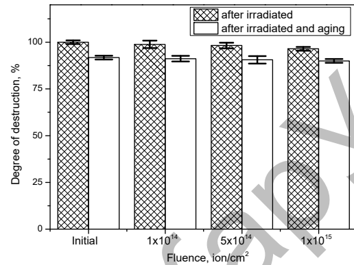
Fig. 7. Diagram of changes in the degree of destruction of ceramics before and after tests.
