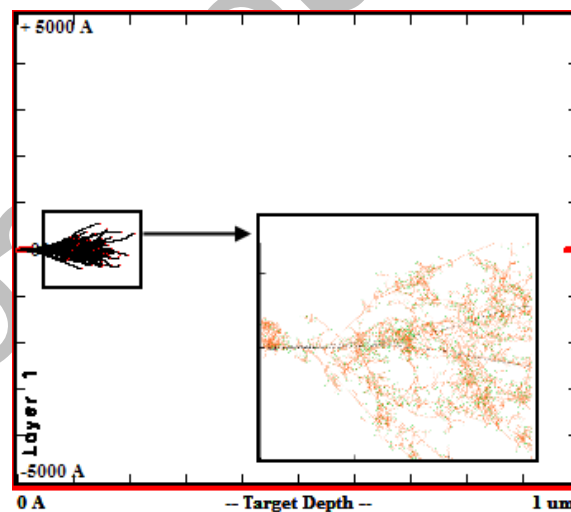
Fig.1. \text{Xe}^{22+} ion paths in SiC ceramics
