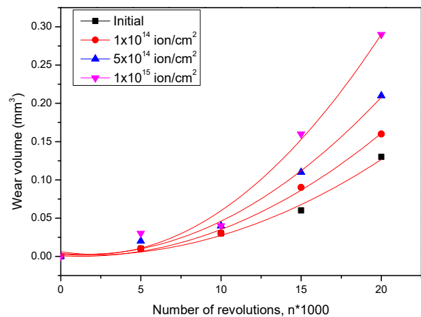
Fig.4. The dynamics of changes in volume loss during wear, depending on the dose.
