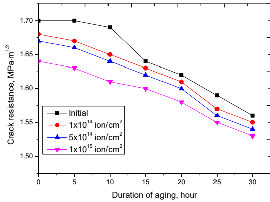
Fig. 6. A graph of the dependence of the crack resistance on the aging time of the samples before and after irradiation.
