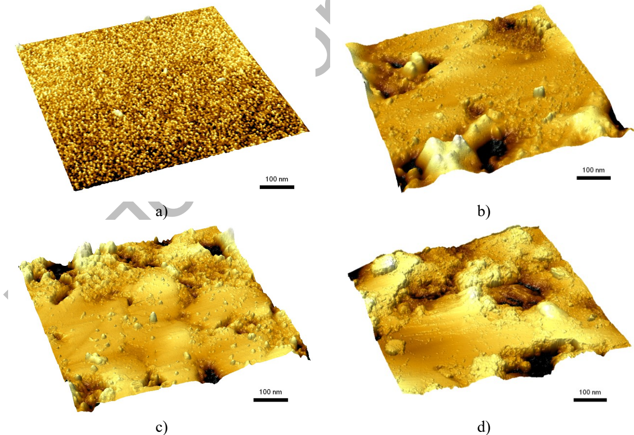
Fig.2. 3D atomic force microscopy (AFM) images of ceramics before and after irradiation: a) Initial sample; b) 10^{14} ion/cm 2 ; c) 5 \times 10^{14} ion/cm 2 ; d) 10^{15} ion/cm 2
