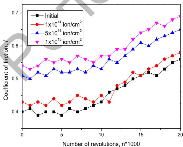
Fig.3. Dependence of the coefficient of dry friction on the dose.
