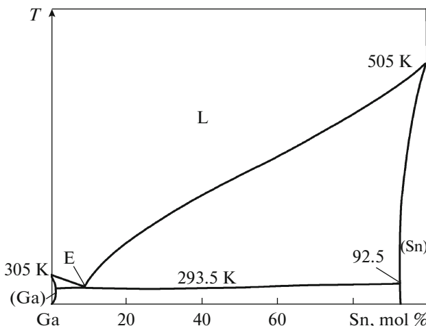
Fig. 1. Ga–Sn phase diagram [10].
