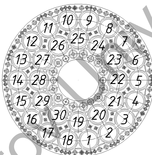
Fig. 1. The cartogram of the WCTC layout in the reactor core
