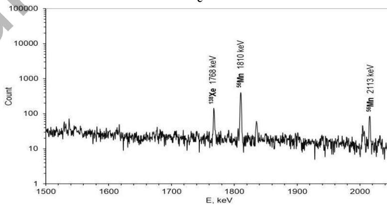
Fig. 2. Gamma spectrum of the IVG.1M reactor coolant:
