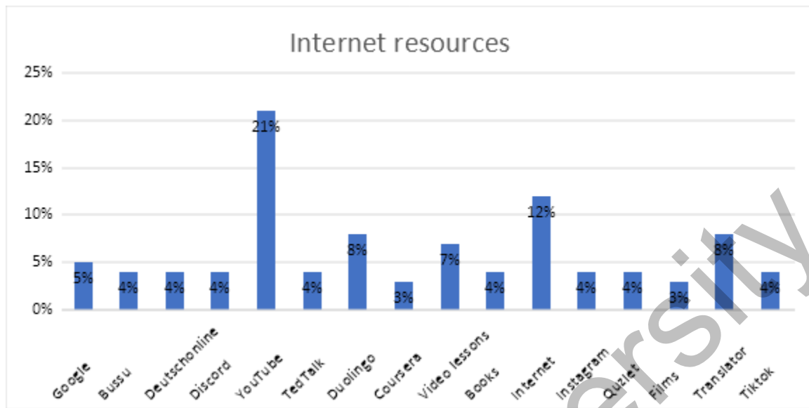
Figure 9. Internet resources
