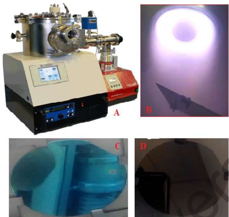
Figure 2. The process of forming the Mn_4Si_7 coating by the method of magnetron sputtering
