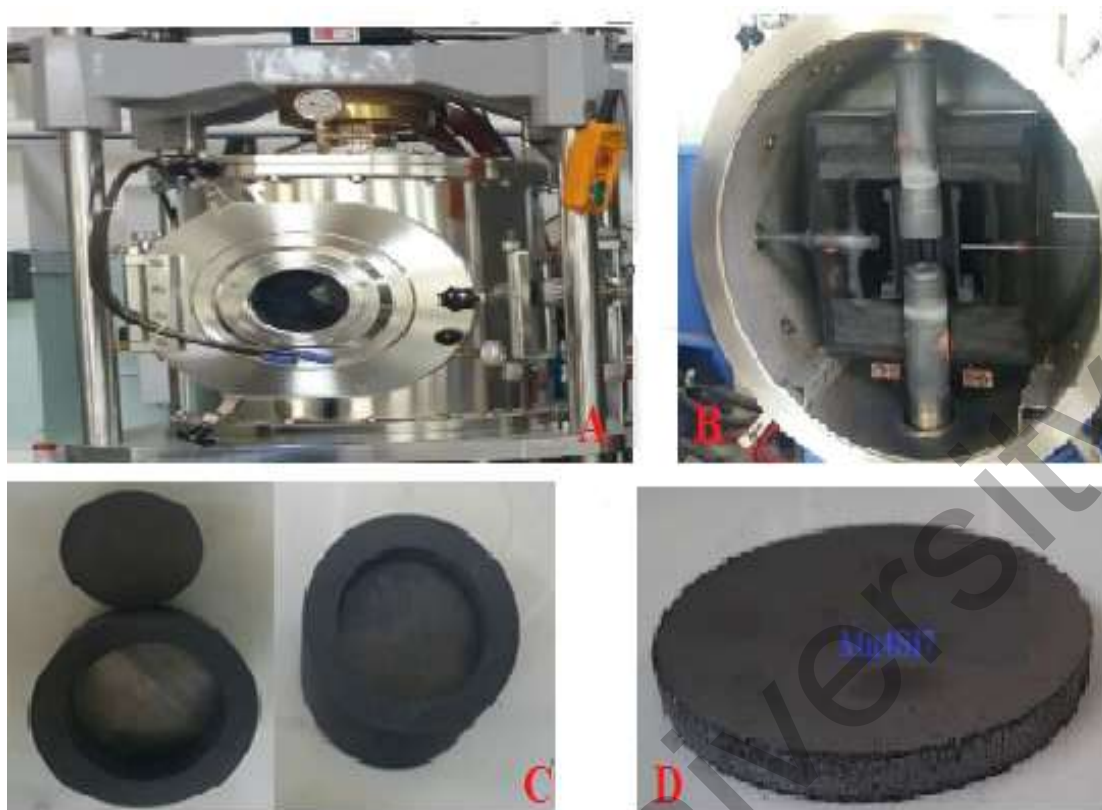
Figure 1. Preparation of the \text{Mn}_4\text{Si}_7 target by the (SPS) method
