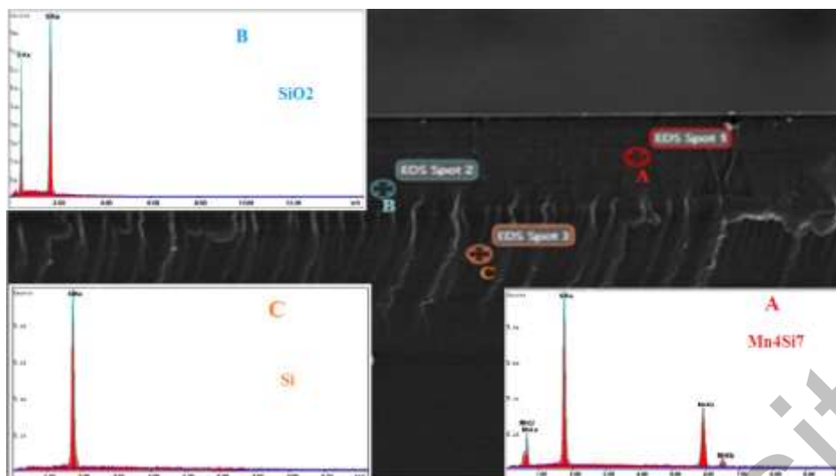
Figure 3. Image of Mn_4Si_7 sample (Scios FEI; Quanta 200 3D)
