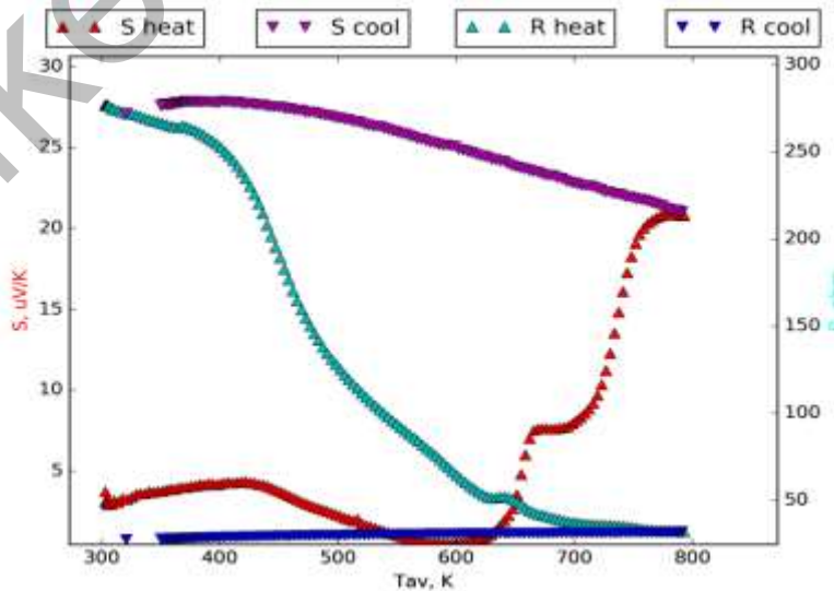
Figure 7. Temperature dependence of the Seebeck coefficient ( S ) and resistance ( R ) of a thin Mn 4 Si 7 coating
