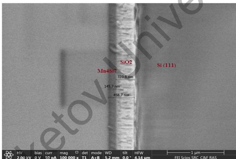
Figure 4. Image of nanosized Mn_4Si_7 coating on SiO_2/Si structure
