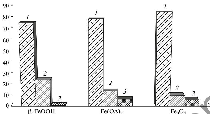
Fig. 5. Ratios between the products of hydrogenation and hydrogenolysis in the presence of the nanocatalysts \beta -FeOOH, Fe(OA) 3 , and Fe 3 O 4 : (1) hydrogenation products, (2) degradation products, and (3) unreacted substances.
