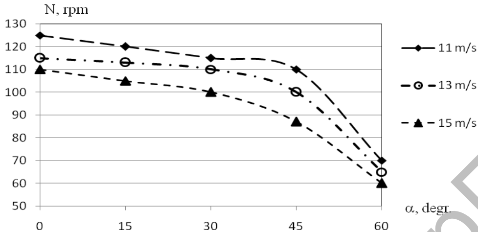
Fig.4. Dependence of rotation frequency on the yaw angle of the flow \alpha at three different flow rates
