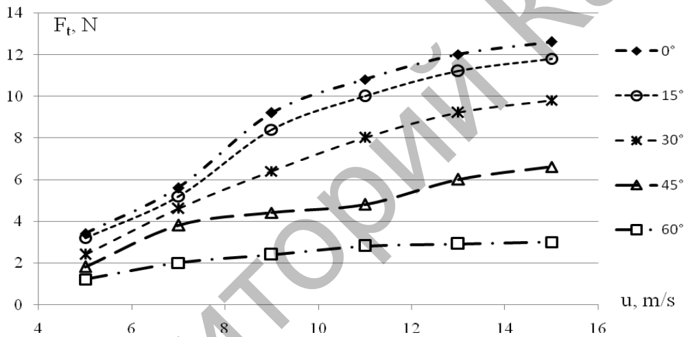
Fig.5. Dependence of the tractive force of wind turbine model at different yaw angles of the flow
