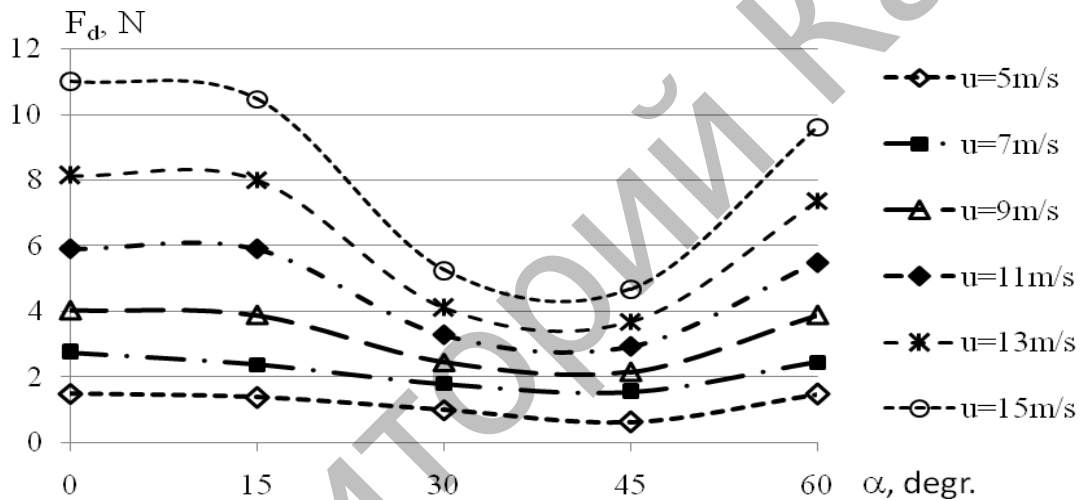
Fig.3. Dependence of the drag force on the yaw angle of the flow \alpha at different flow rates.
