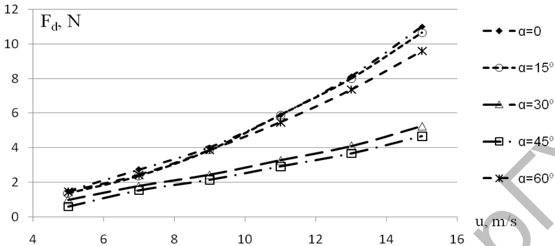
Fig.2. Dependence of the drag force on the flow rate at different yaw angles of the flow \alpha
