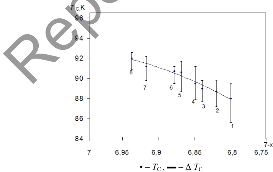
Figure 3. Dependences of superconducting parameters of the films on oxygen stoichiometry
