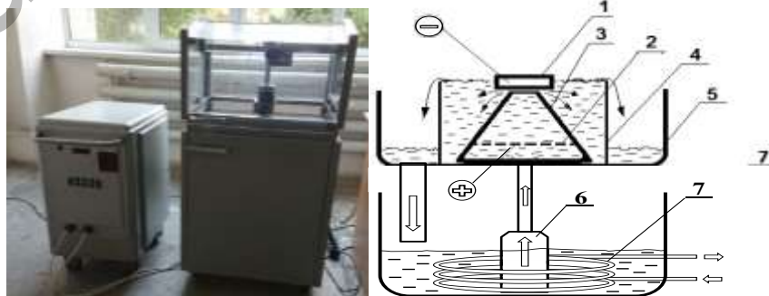
1 — sample to be treated (cathode), 2 — stainless steel anode with holes, 3 — cone-shaped partition, 4 — working chamber — bath with electrolyte, 5 — pan, 6 — pump, 7 — heat exchanger
