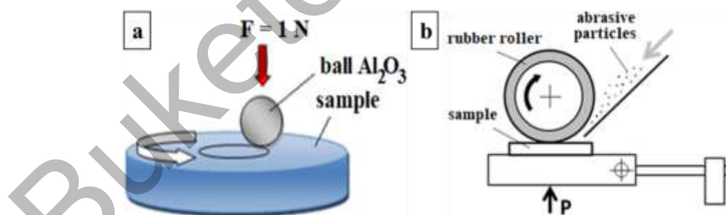
a — according to the scheme “ball on disk”, b — according to the scheme “rotating roller — plane surface”
