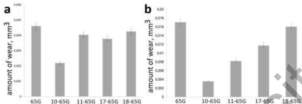
Figure 5. Data on the wear volume of samples after test with counterbodies of \text{Si}_3\text{N}_4 (a) and 100Cr6 (b)
