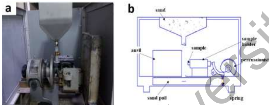
Figure 3. Experimental bench for shock-abrasive wear according to GOST 23.207-79
