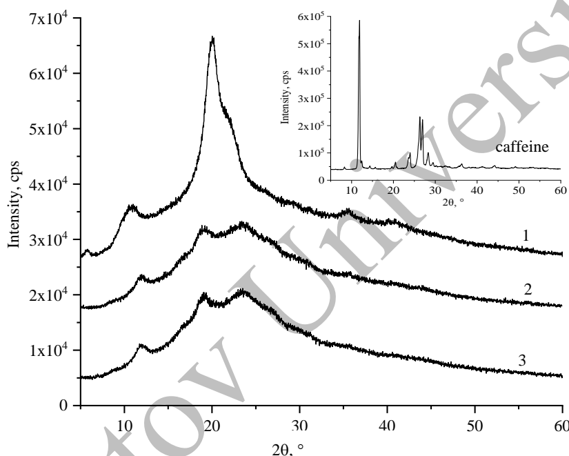
Figure 4. X-ray diffraction patterns of the sample 1 (1), sample 2 (2), and chitosan (3)
