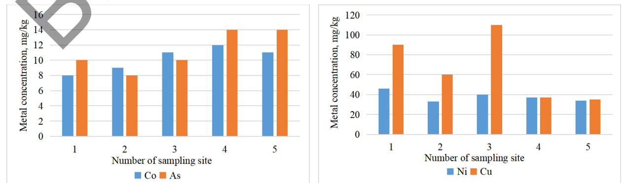
Figure 6. Concentration of heavy metals in solid snow sediment at different distances from the Pavlodar Petrochemical Plant
