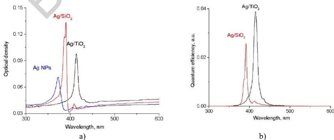
Fig. 4. Calculated absorption (a) and quantum efficiency (b) spectra of Ag and core/shell NPs.
