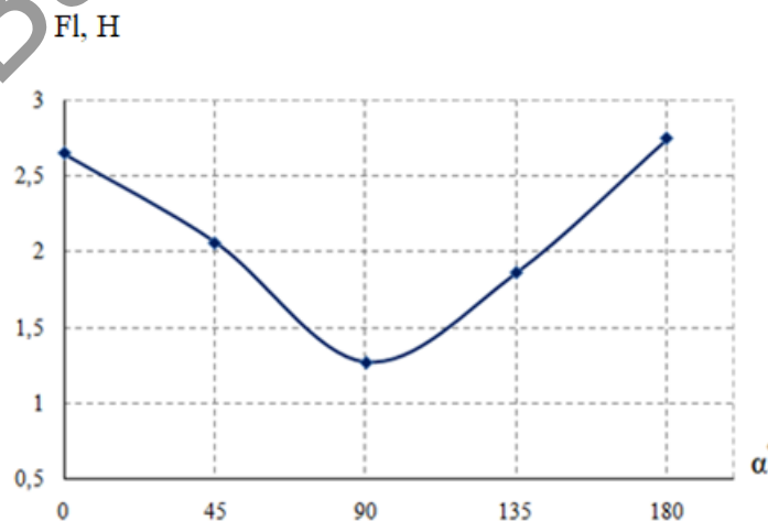
Figure 4. The results of lifting force measurements depending on the angle of inclination at a flow rate of 5 m/s
