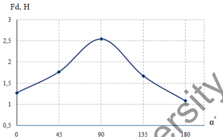
Figure 3. The results of measurements of the drag force from the angle of inclination at a flow rate of 5 m/s
