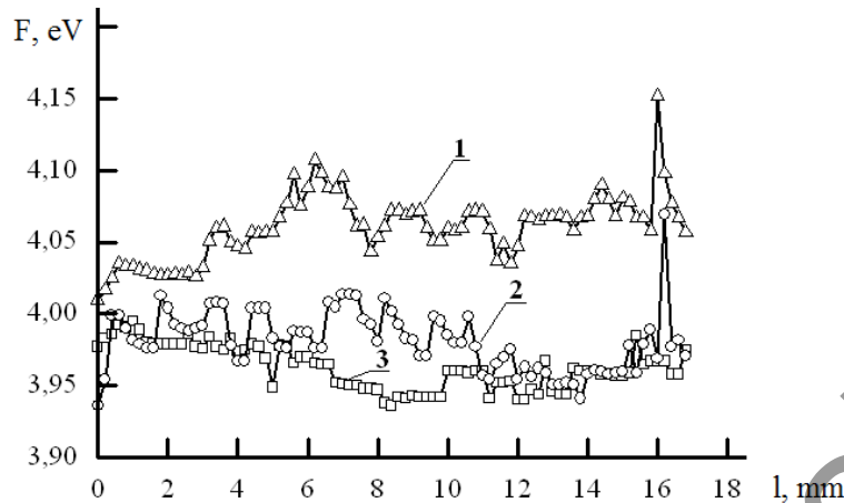
Fig.2. Distribution works of electron output along the surface of standards from the steel 60S2A after a wear with different amplitude of the transversal slipping: (1) A_{trs} = 0 mm; (2) A_{trs} = 0.06 mm; (3) A_{trs} = 0,2 mm.
