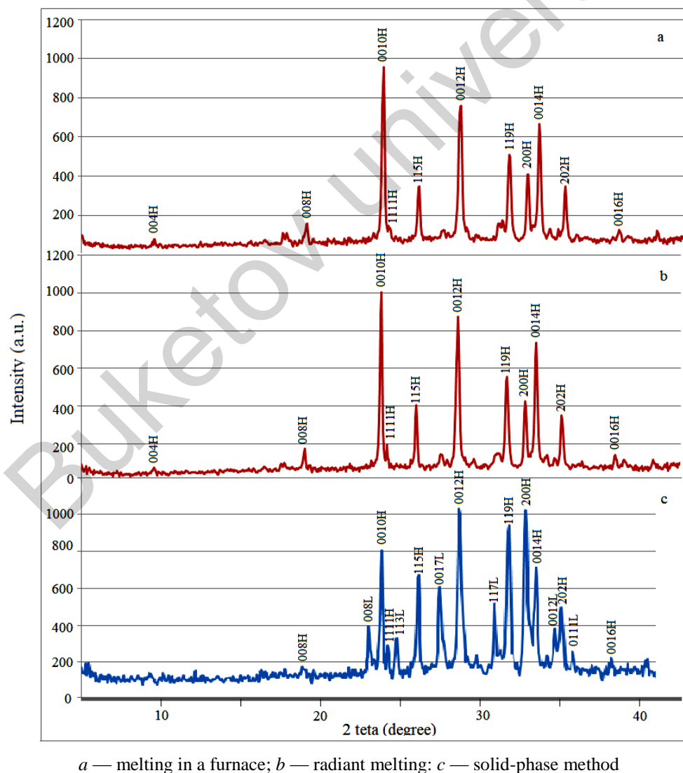
Figure 4. Diffractograms of HTSP samples of composition \text{Bi}_{1.6}\text{Pb}_{0.4}\text{Sr}_2\text{Ca}_2\text{Cu}_3\text{O}_y after heat treatment at 850 °C, 96 hours
