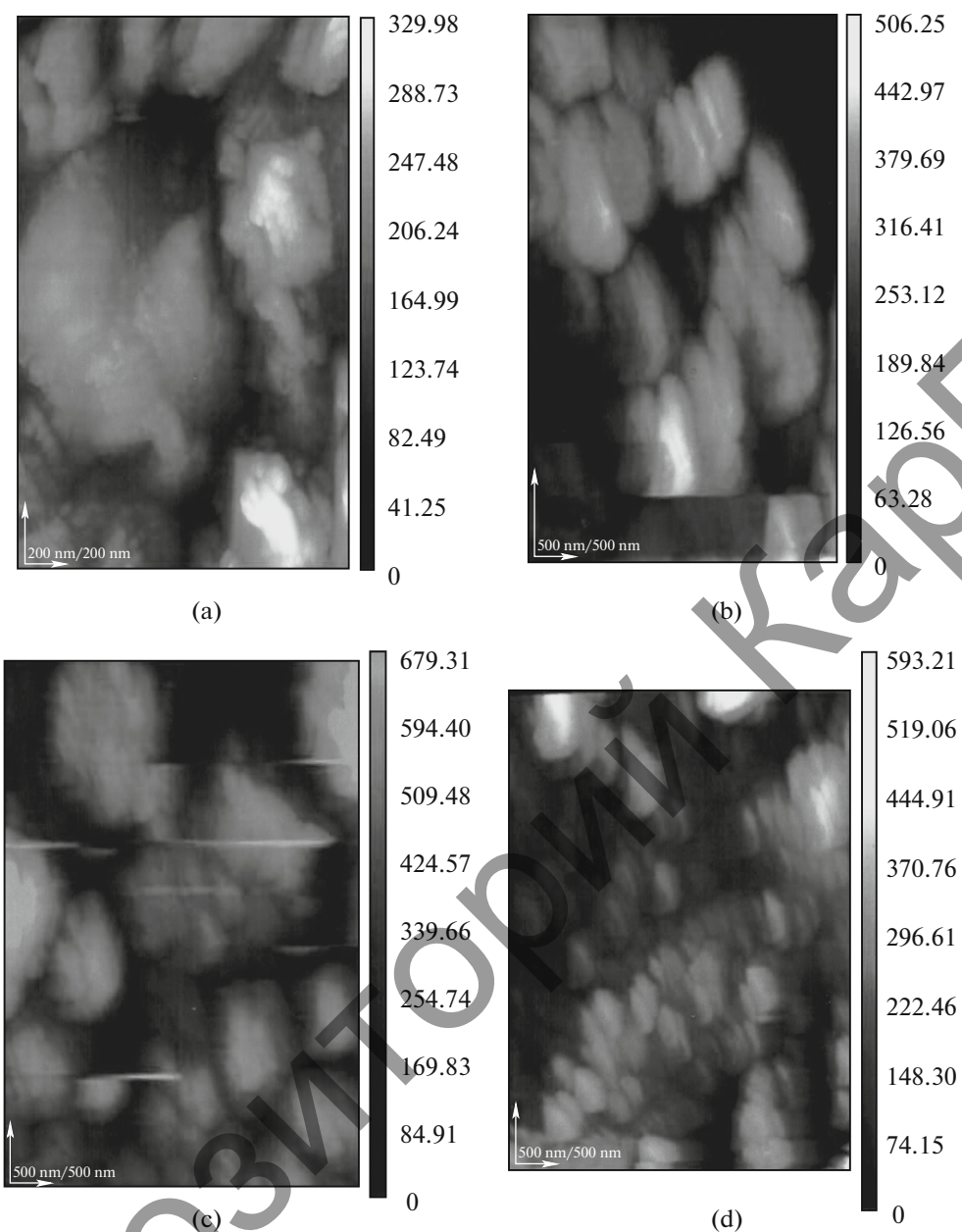
Fig. 1. Electronic microimages of nanosized (nanocluster) ferro-chromo-manganites \text{LaM}_{0.5}\text{FeCrMnO}_{6.5} ; (a) \text{M}^{\text{II}}\text{-Mg} , (b) Ca, (c) Sr, and (d) Ba.
