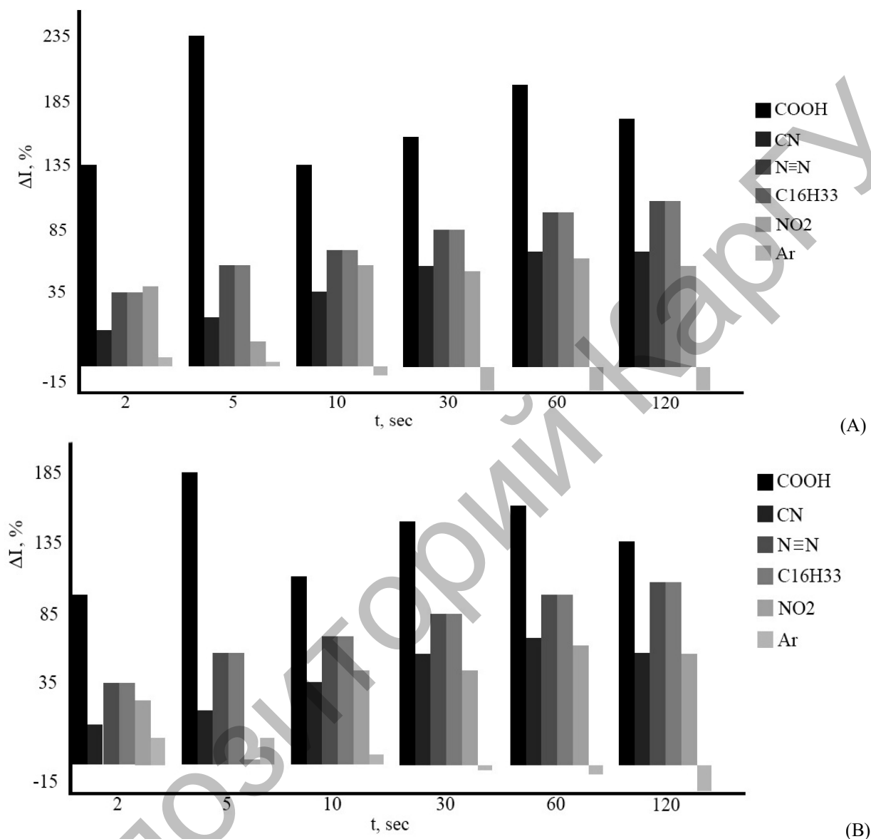
A — cathode currents; B — anode currents. The background electrolyte is \text{KCl } 0.5 \text{ M} ; scan rate 80 \text{ mV}\cdot\text{s}^{-1} ; concentration 10 \text{ mg}\cdot\text{l}^{-1}
