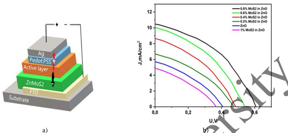
Fig.6. a) the architecture of the inverted PSC b) J–V characteristics of inverted solar cells
