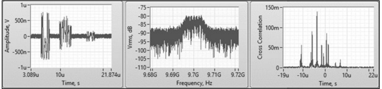
Fig.2. Result of simulation of the PRSS signal at the receiving point:
