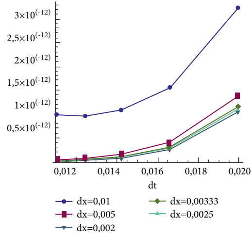
FIGURE 5: Relative errors of the numerical solution.
