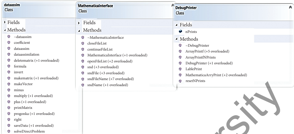
FIGURE 6: Class diagram of the concentration calculation module.
