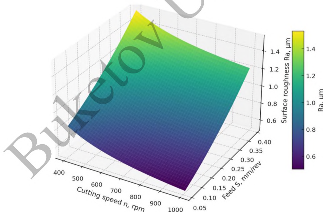
Fig. 2. Dependence of surface roughness R_a on speed n and feed S (the 3D graph shows the minimum R_a values in the range of high speeds and low feeds)
