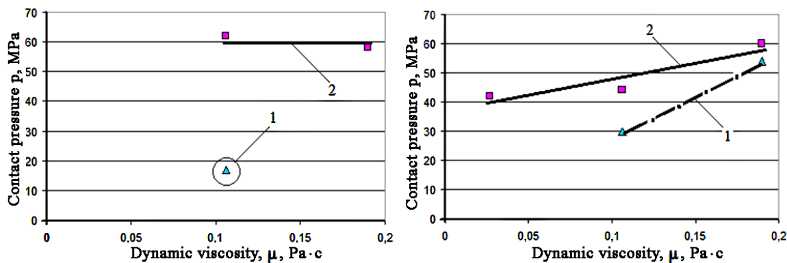
a) at v_2 = 5.08 \pm 0.6 mm/s; b) at v_1 = 10.16 \pm 0.8 mm/s; 1) steel 45 when borated; 2) with boron carburizing steel 45
