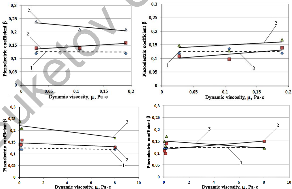
a, b) at v = 5.08 \pm 0.6 mm/s; c, d) at v = 10.16 \pm 0.8 mm/s; 1) steel 45 is not modified; 2) "steel 45 + BC"; 3) "steel 45 + B"
