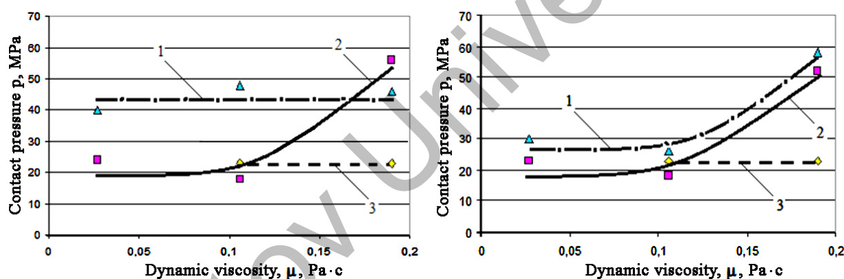
a) at v_2 = 5.08 \pm 0.6 mm/s; b) at v_1 = 10.16 \pm 0.8 mm/s; 1) steel 45 when borated; 2) with boron carburizing steel 45; 3) steel 45 without modification
