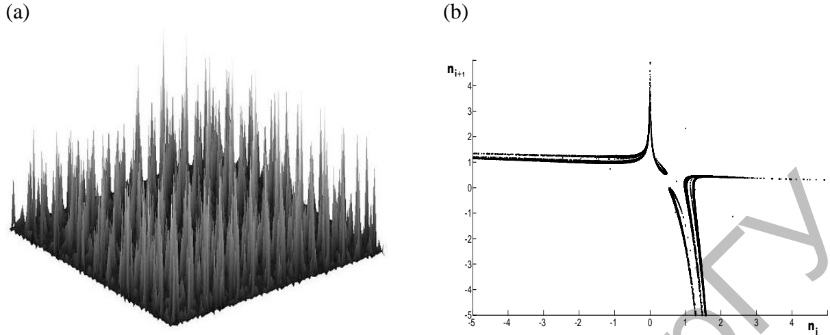
Fig.1. Model of a surface containing vertical quantum nanowires (a) and its phase plane (n_i, n_{i+1}) (b). n_0 = p_0 = 0.25 , a_0 = 1.7 C_n = C_p = C_a = 0.999 , \gamma_n = \gamma_p = \gamma_a = 2 + I_1 , \tau = 10 .
