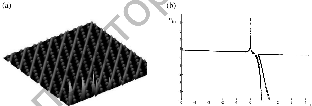
Fig.4. Model of a surface containing horizontal quantum nanowires (a) and its phase plane (n_i, n_{i+1}) (b).
