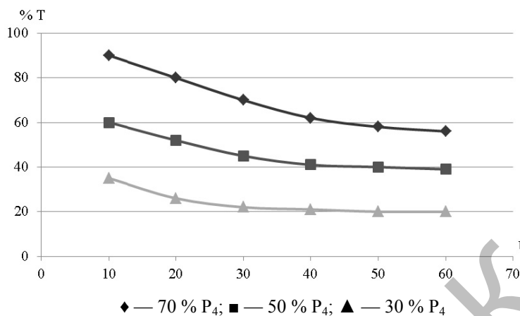
Figure 3. Dependence of the combustion time on the initial voltage of the generator
