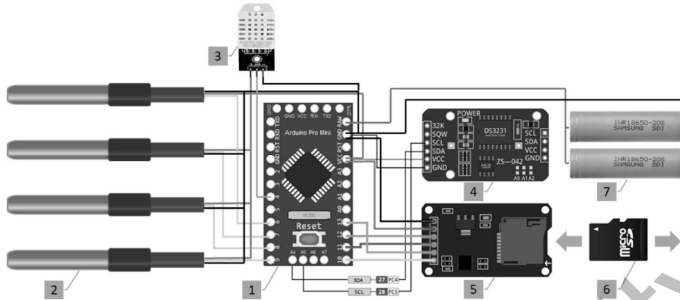
Fig. 1. MSD IT-architecture
