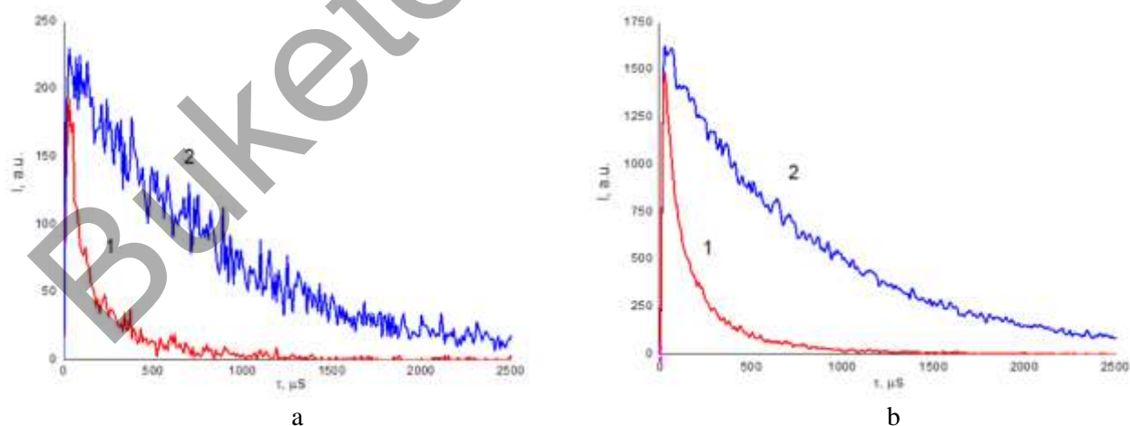
Figure 3. Decay kinetics of BR Phos on glass (a) and on SIFs (b) with (1) oxygen and (2) without it ( \lambda_{ex} = 530 nm)
