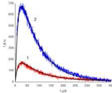
Figure 5. Decay kinetics of singlet oxygen phosphorescence ( \lambda_{reg} = 1270 nm), sensitized with BR, on glass (1) and on SIFs (2) at atmospheric pressure ( \lambda_{ex} = 530 nm)
