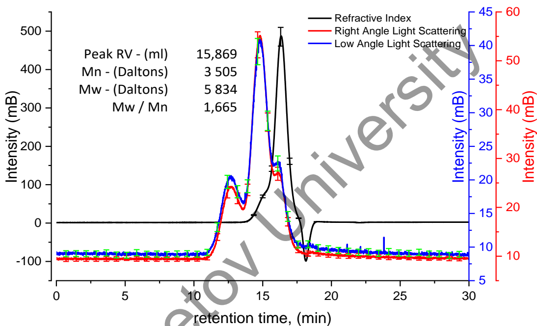
Figure 1. Molecular mass of the final product of PEGF obtained after 8 hours of polycondensation
