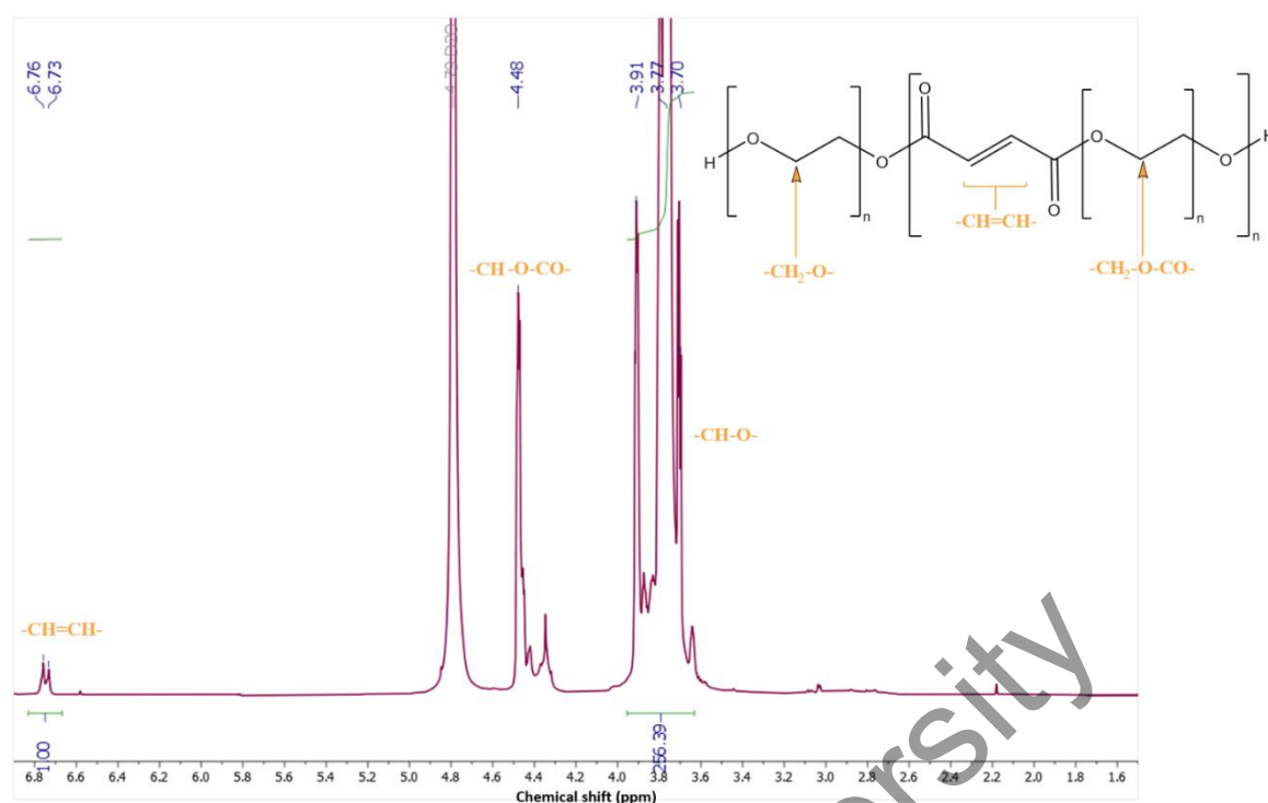
Figure 5. ^1\text{H} NMR-spectra of PEGF obtained after 8 h of polycondensation
