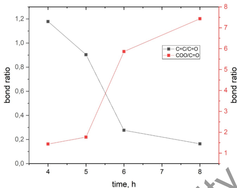
Figure 3. The dependence of the ratio of number of double bonds -C=C- and carboxylic groups -COO- to the -C=O bonds in chemical structure of PEGF, obtained at different time of polycondensation of PEG-600 and fumaric acid
