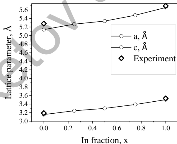
Figure 1. Calculated lattice parameters of \text{In}_x\text{Ga}_{1-x}\text{N} within LDA in comparison with experimental values [35, 53]
