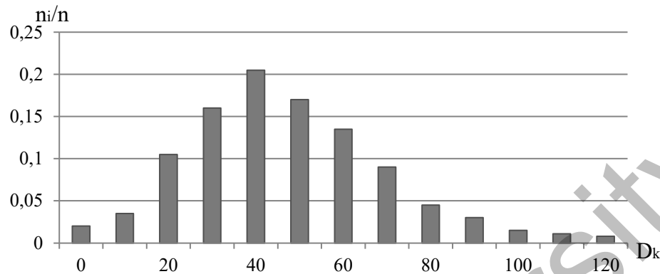
Fig. 6. The size distribution of sludge particles after treatment with an electric discharge pulse of average power.
