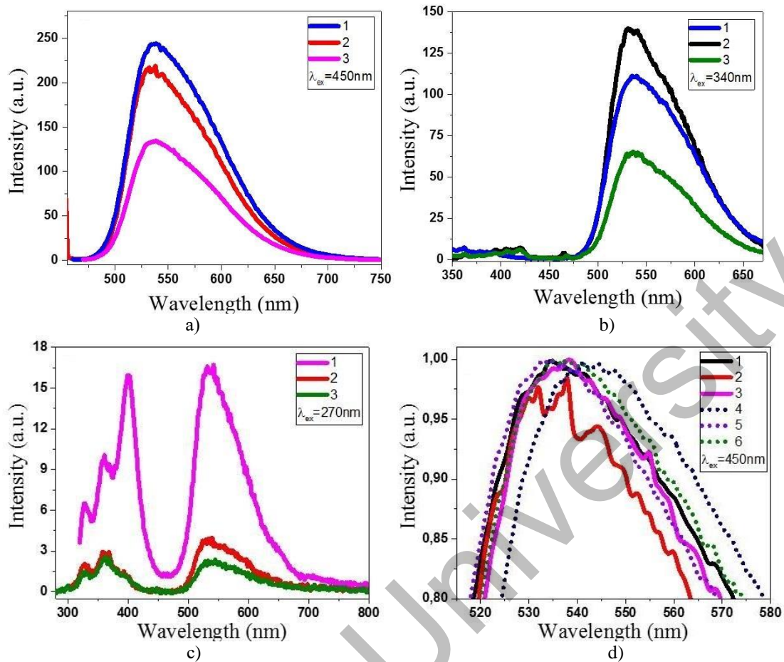
Fig 5. Luminescence spectra of the synthesized samples upon excitation at: a) 450 nm, b) 340 nm, c) 270 nm, d) 450 nm.
