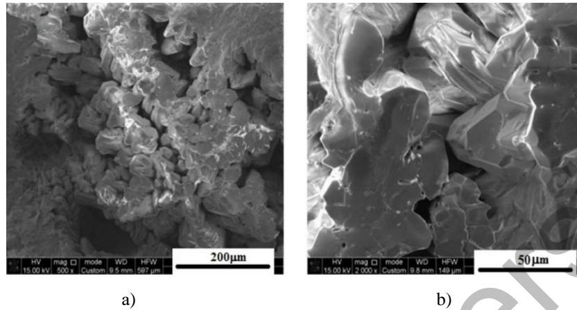
Fig 3. SEM images of the cleavage site for sample 4 (YAG:Ce, Gd) at different magnification
