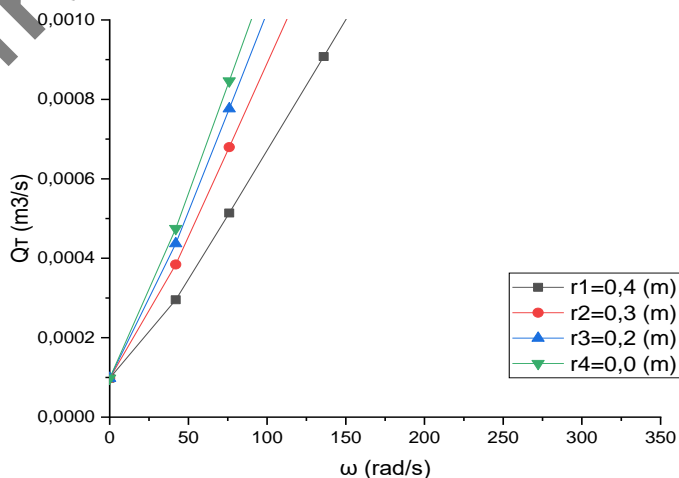
Figure 4. The total theoretical flow of liquid through the throttle hole with a diameter of 3.0 mm, at different positions of the liquid ring
