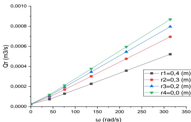
Figure 2. Total theoretical fluid flow through a 1.5 mm diameter choke hole, at different positions of the fluid ring
