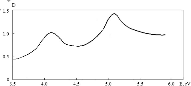
Figure 5. Crystal absorption spectrum \text{K}_2\text{SO}_4\text{-Ni}^{2+} , measured at ambient temperature
