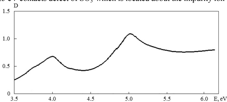
Figure 3. \text{K}_2\text{SO}_4\text{-Mn}^{2+} crystal absorption spectrum +, measured at ambient temperature
