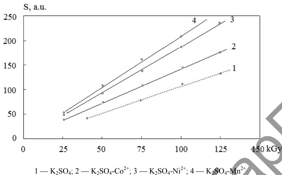
Figure 7. The dependence curves of speeds of accumulation lightsum on the radiation dose in TSL peak at the temperature 190 K
