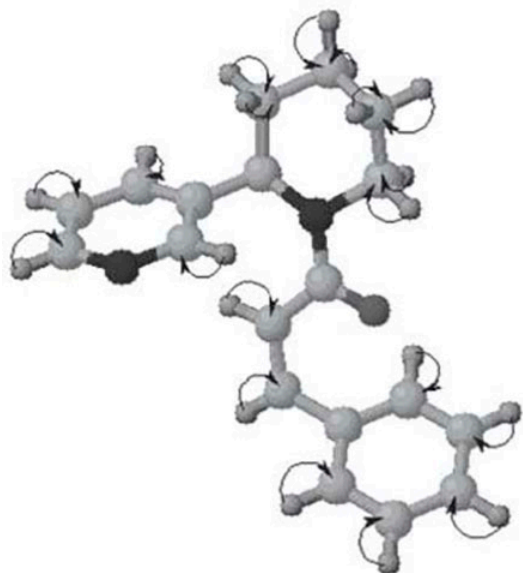
Fig. 1. Correlations in the HMQC spectrum of compound 1.
