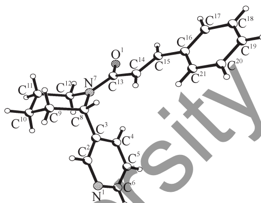
Fig. 2. General view of compound 1 molecule in the crystal.
