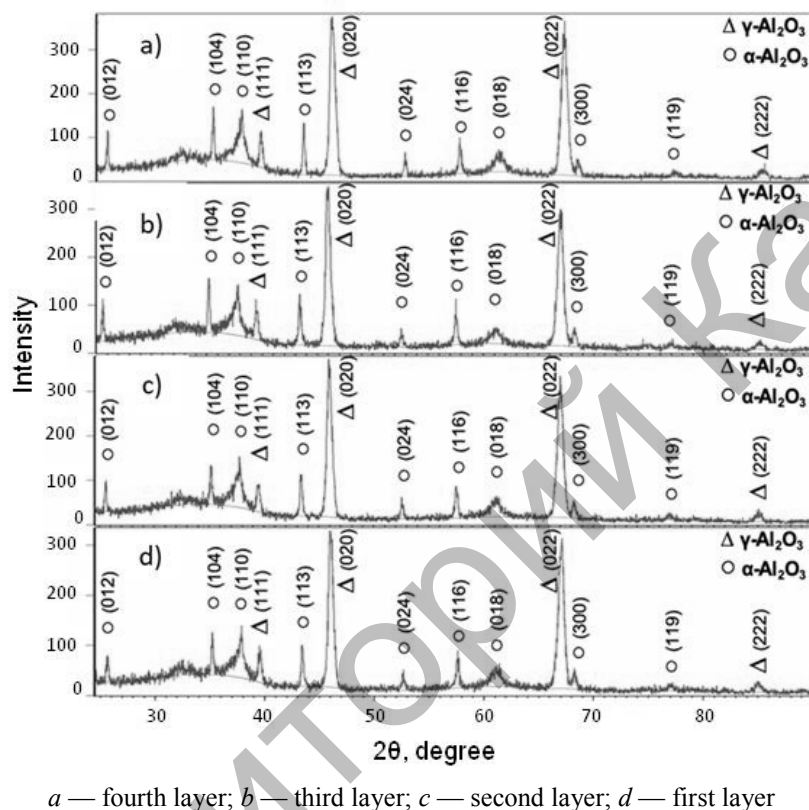
Figure 2. Diffractogram of the coating
