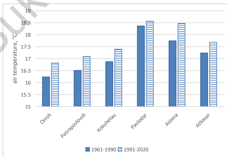
Figure 1. Air temperature of the vegetation period (may-august) for the basic (1961–1990) and modern periods (1991–2020) with averaged data for 30 years.
