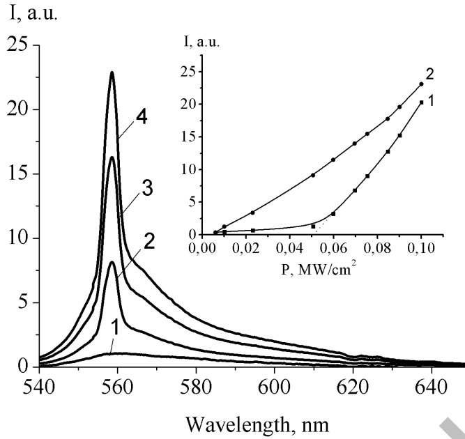
Fig.3. Emission spectra of aqueous solution of R6G at different pump power density: 1 - 0.01; 2 - 0.03; 3 - 0.04; 4 - 0.05 MW/cm 2 . The inset shows the emission intensity on the pump energy: 1 - pure dye solution; 2 - R6G solution with 4 \cdot 10^{-4} mol \cdot l -1 NP Ag.
