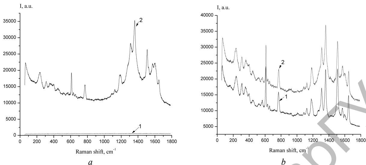
Figure 3. SERS spectra of Rh6G ( 10^{-4} M) on composite II (a, 2), composite I (b, 2), on AgNPs (b, 1) and Raman spectrum of Rh6G on glass (a, 1) excited at 632.8 nm
