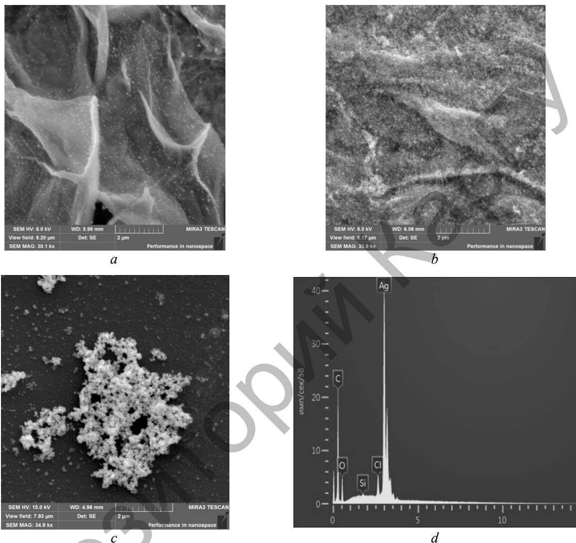
a-c — composite I, composite II, colloidal Ag NPs, respectively; d — energy-dispersive X-ray analysis spectrum of composite II
