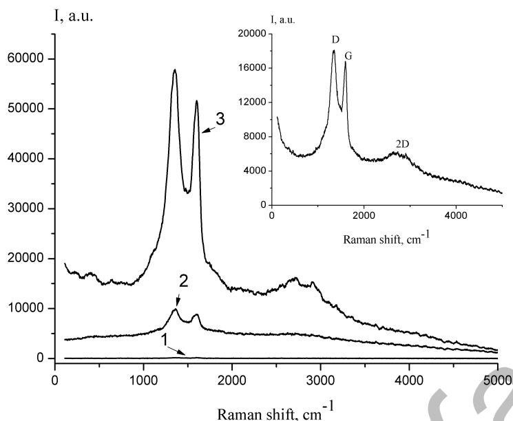
Figure 2. Raman spectra of the GO (1) and the SERS spectrum of composite I (2, 3) ( \lambda_{\text{exc}} is 632.8 nm, laser power on the samples is 1.1 mW). The inset shows the Raman spectrum of the GO at laser power of 35 mW
