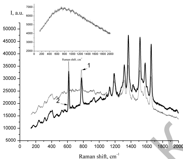
Figure 5. SERS spectra of Rh6G ( 10^{-6} M) on AgNPs (1) (laser power on the sample is 0.22 mW) and on composite (2) (laser power on the sample is 0.696 mW). The inset shows the Raman spectrum of Rh6G ( 10^{-6} M) on glass (the laser power on the sample is 0.696 mW)
