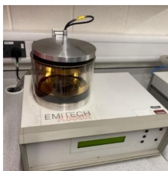
Figure 8. Appearance of the “Emitech K550X” installation
