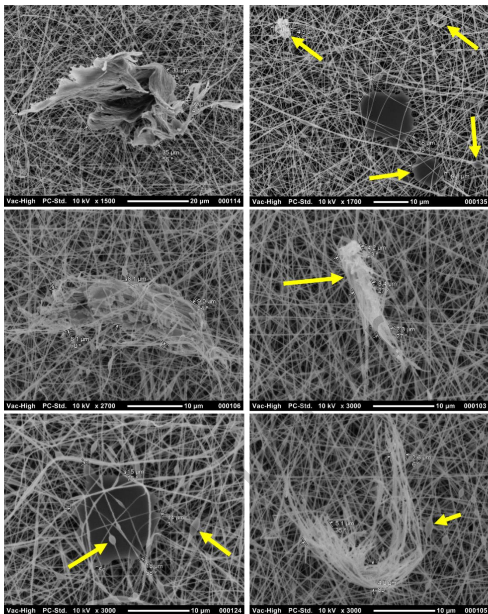
Figure 11. SEM image of defects on the surface of nanofibers at high electrospinning voltage values
