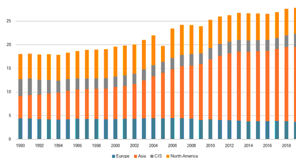
Fig. 2. The share of CO 2 emissions by region of the world for the period 1990–2019
