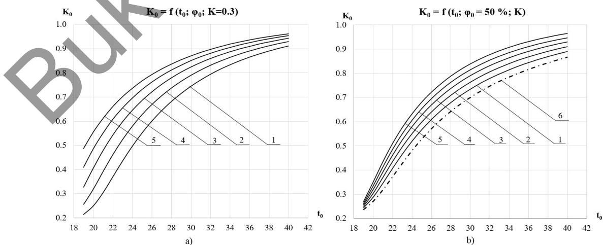
Fig. 4. Graphical relationships between the variable ratio of fresh outside air, the environment parameters and the coefficient K : a) K = 0.3 ; 1-5 – \varphi_0 = 40 - 80\% ; b) \varphi_0 = 50\% ; 1-5 – K = 0.1 - 0.5 ; 6 – K = 0 .
