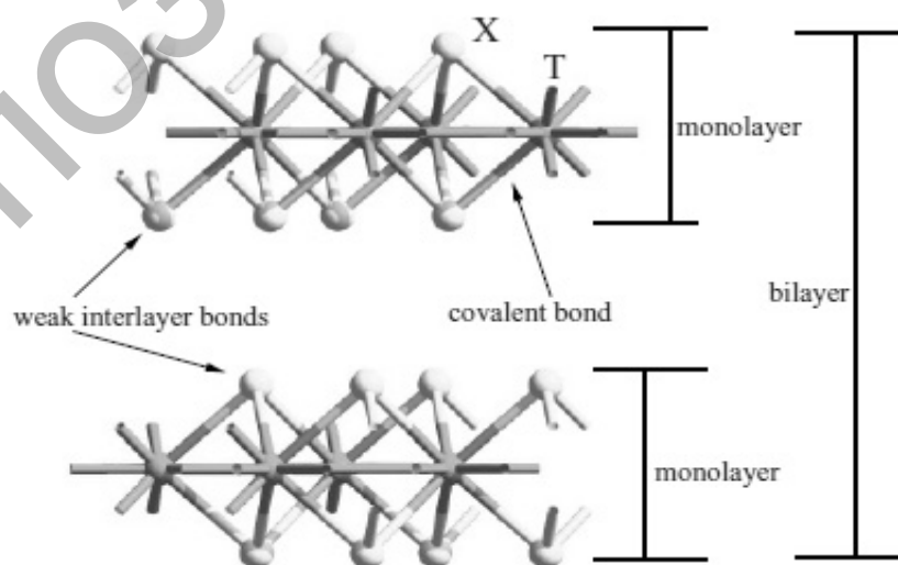
Fig.1. 2D transition metal dichalcogenides.
