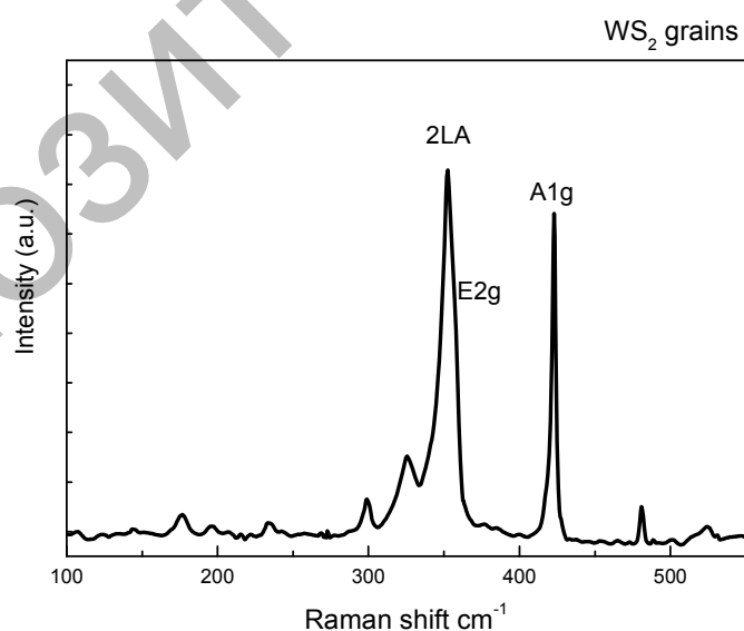
Fig.5. Raman spectroscopy of WS_2 crystal
