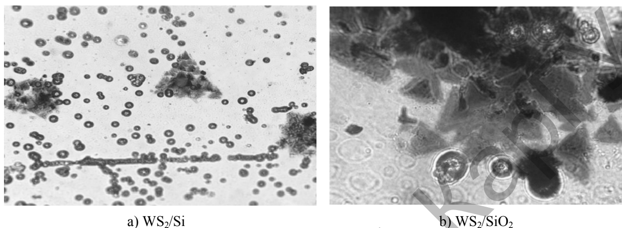
Fig.4. Optical microscope pictures of WS_2 grains: a) onto Si substrate; b) onto SiO_2 substrate
