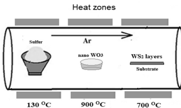
Fig.3. Synthesis of 2-D TMD layers
